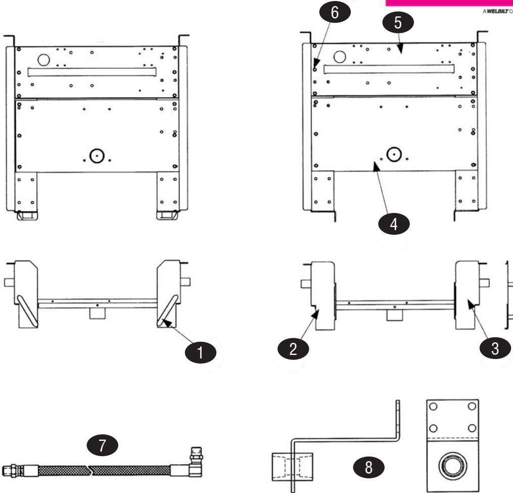
FOOTPRINT III FILTER BASE ASSEMBLIES
