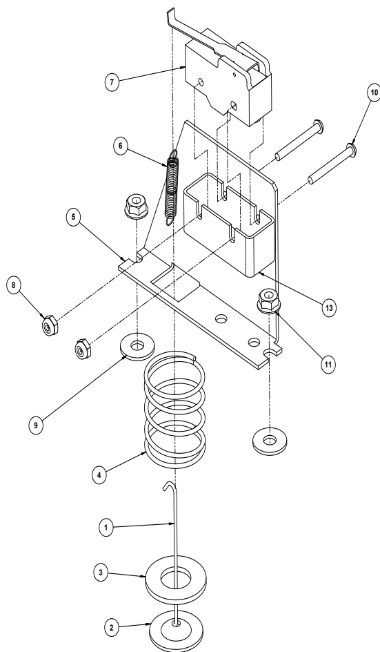
HIGH LIMIT OVERTEMP ASSEMBLY DETAIL VIEW
