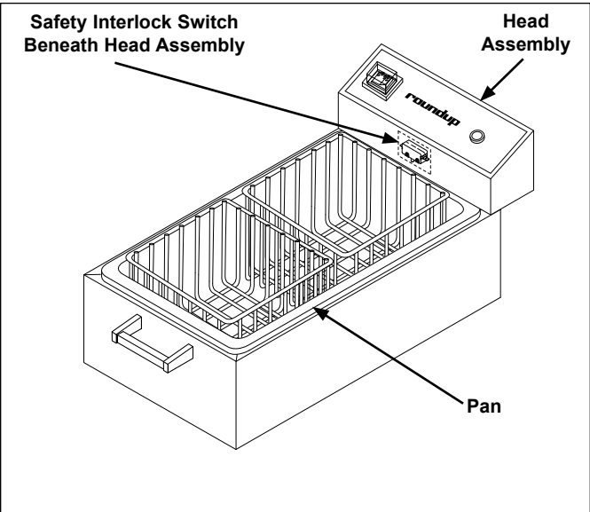
Figure 1. Corn Cooker
