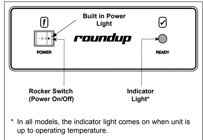
Figure 2. Controls
