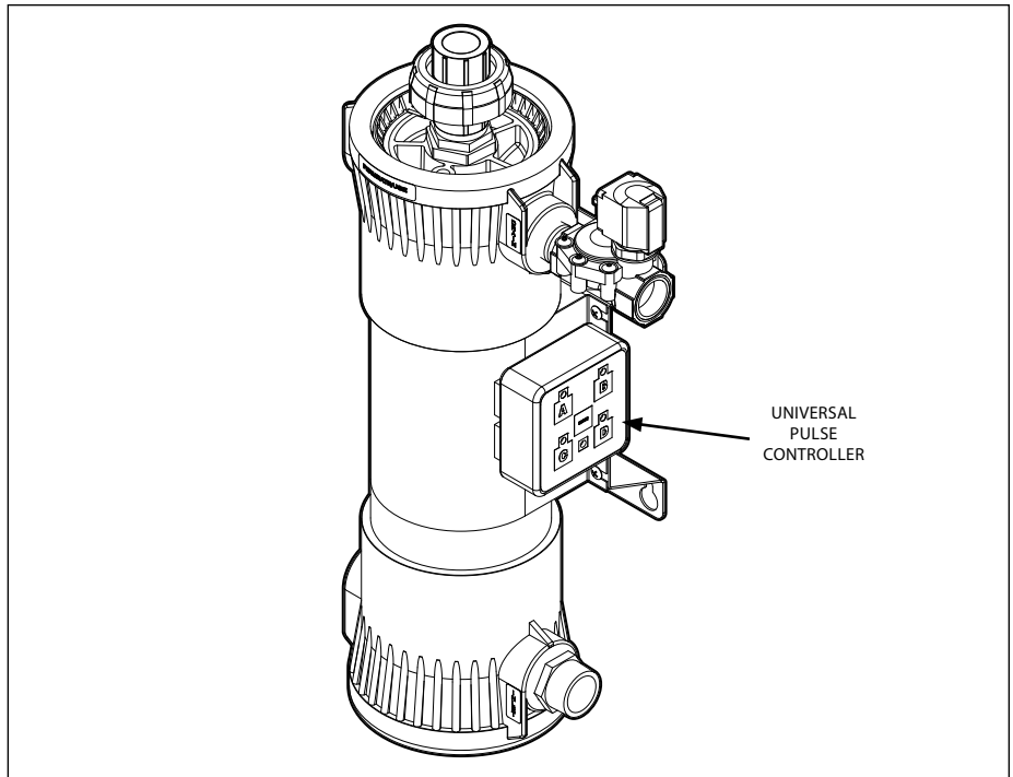
Figure 2. UFL-410 System
