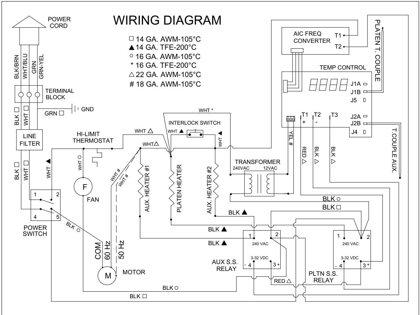
Pictorial Wiring Diagram Heated Base Units
