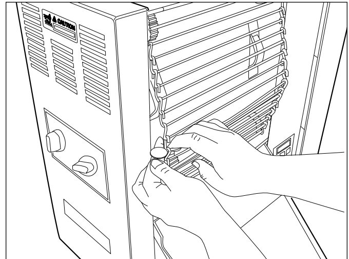
Figure 12. Measuring Conveyor Belt Chain
