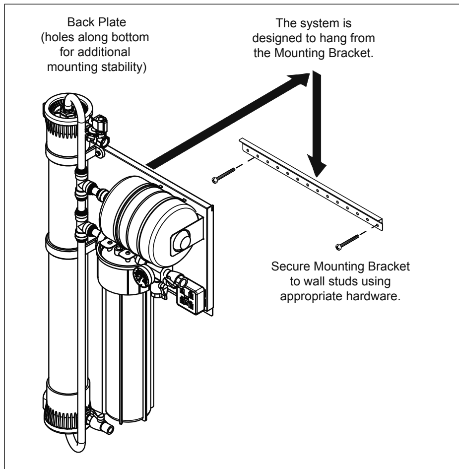
Figure 2. Mounting the System
