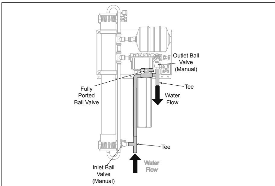
Figure 7. Install Bypass
