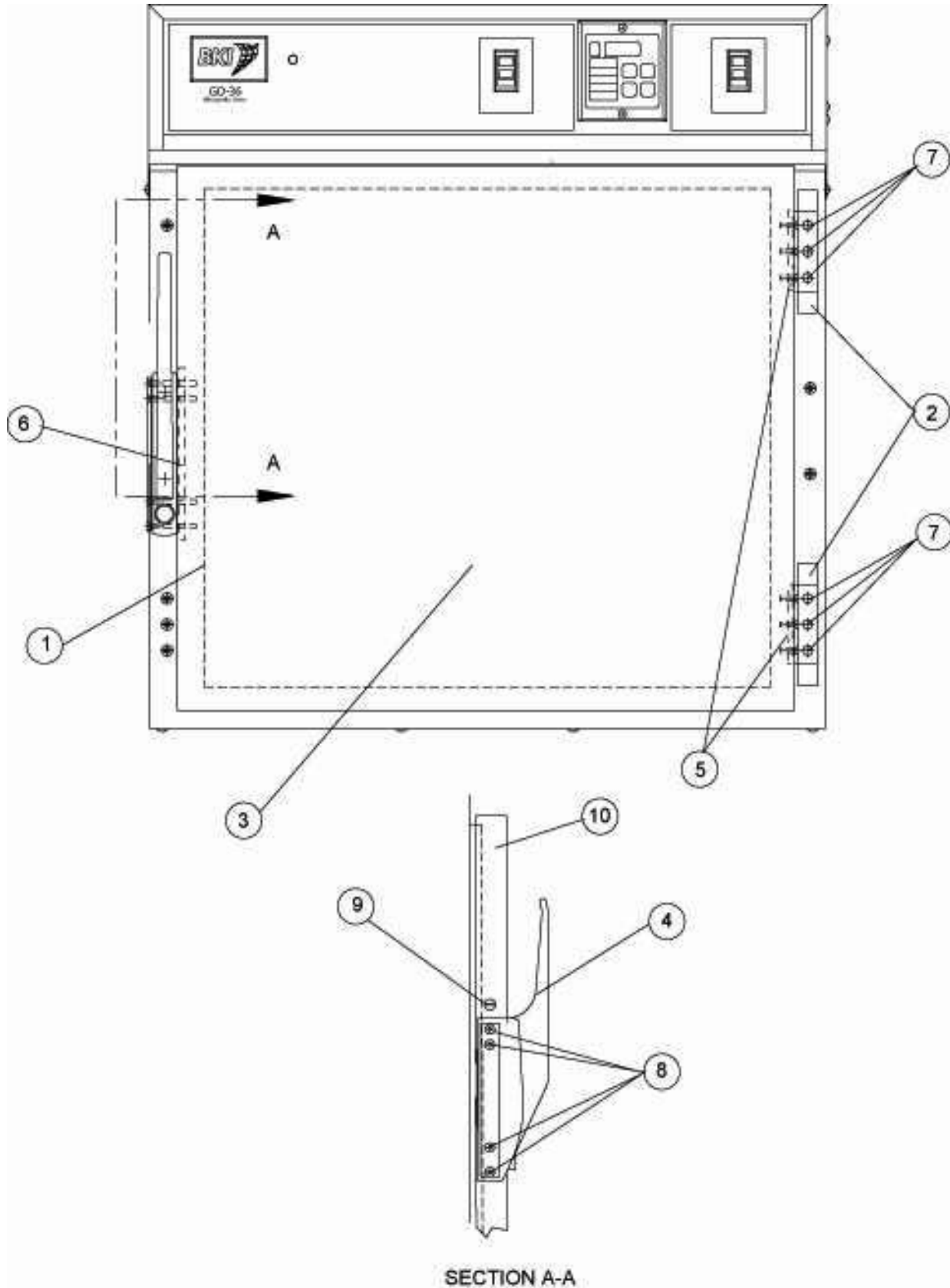
Figure 5. Door Assembly
