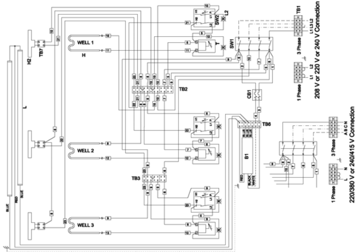
Figure 7. Model SSW-4/CSW-4
