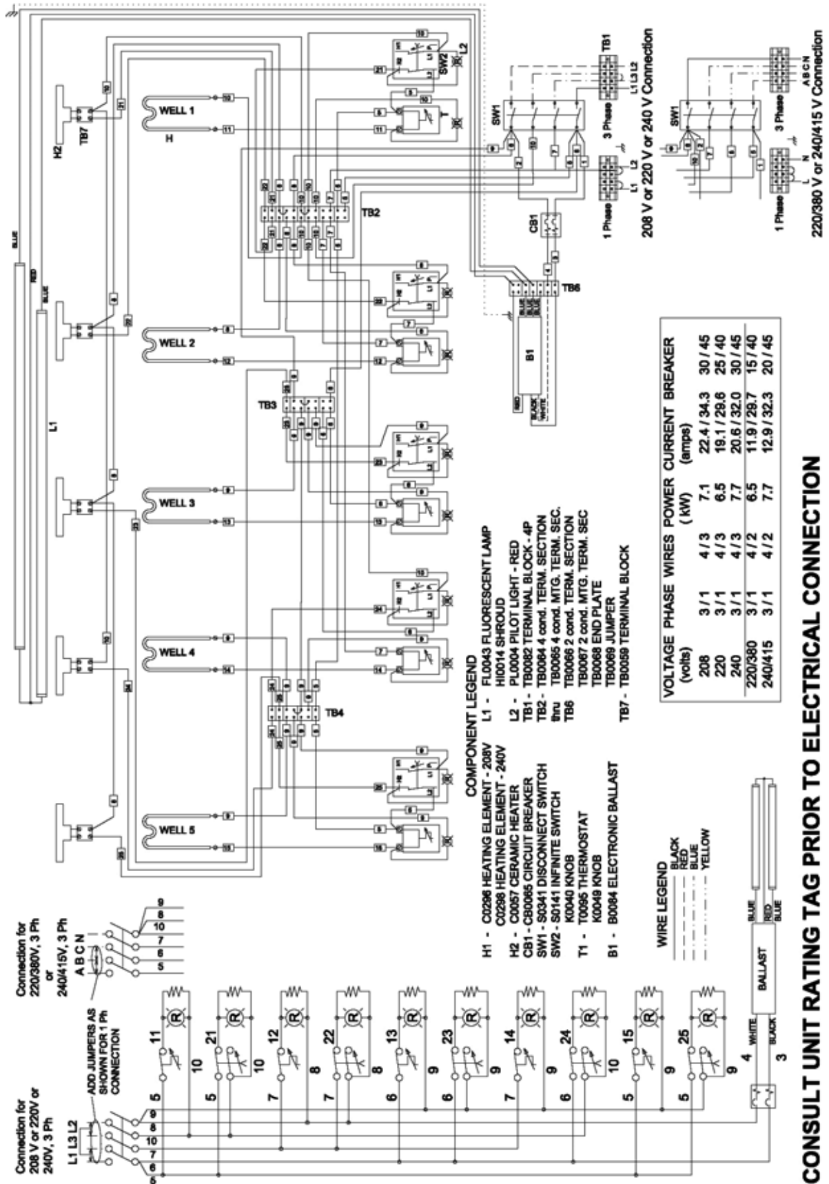
Figure 8. Model SSW-6/CSW-6
