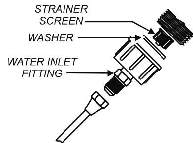
Fig. 14 Clean Strainer Screen
