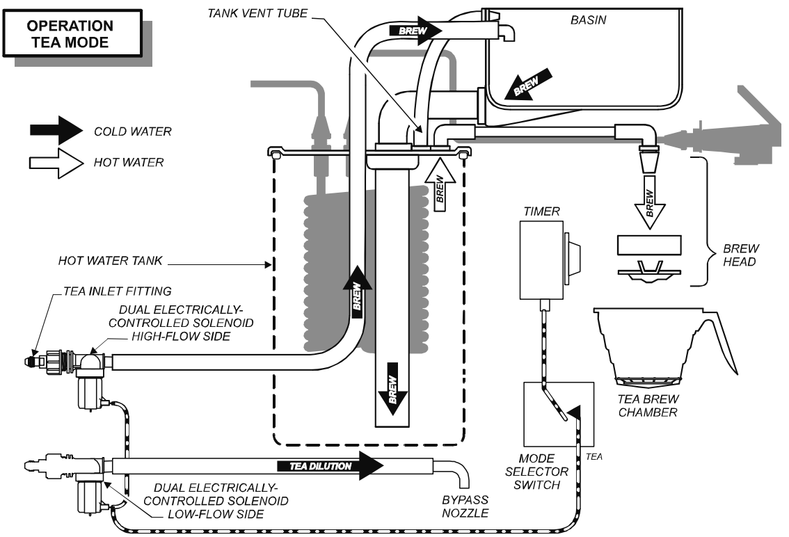
Fig. 3 Brewer Operation Diagram
