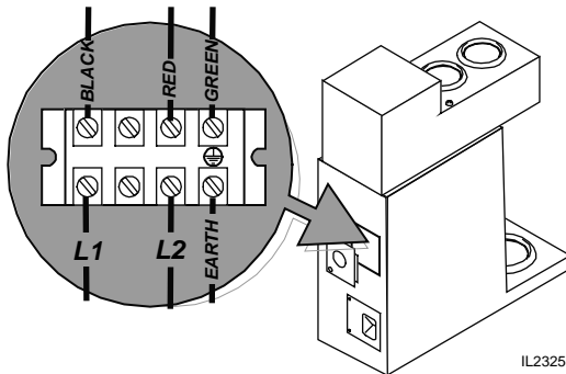
Fig. 3 Wiring Connections
