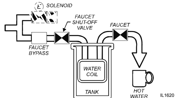
Fig. 6 Water Flow Diagram
