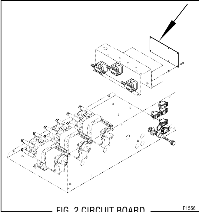
FIG. 2 CIRCUIT BOARD
