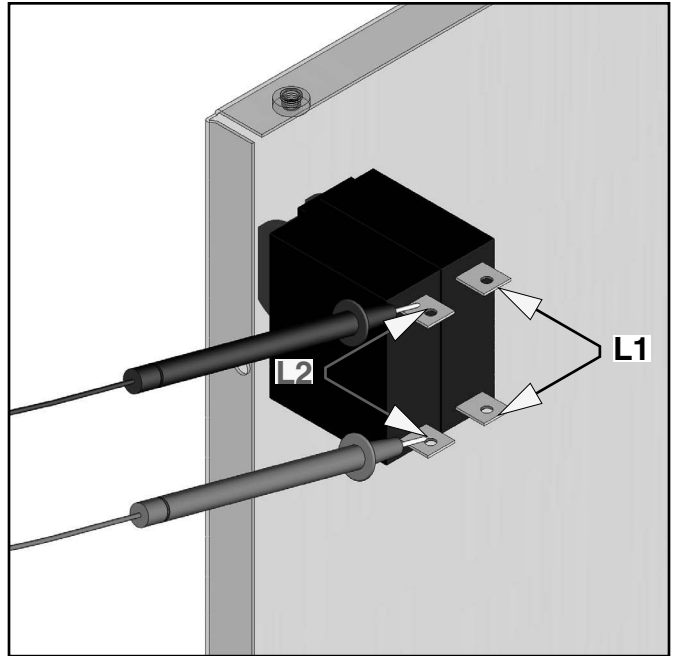
FIG. 22-2 ROCKER SWITCH
