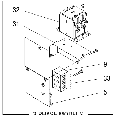
3 PHASE MODELS
