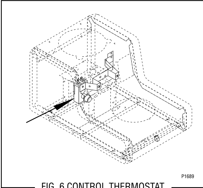
FIG. 6 CONTROL THERMOSTAT
