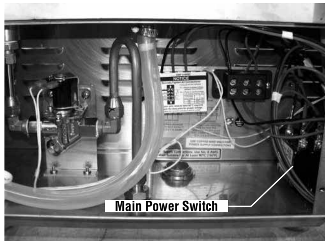
FIG 7 MAIN POWER SWITCH
