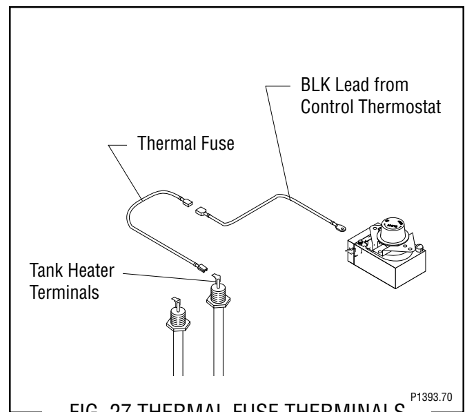
FIG. 27 THERMAL FUSE THERMINALS
