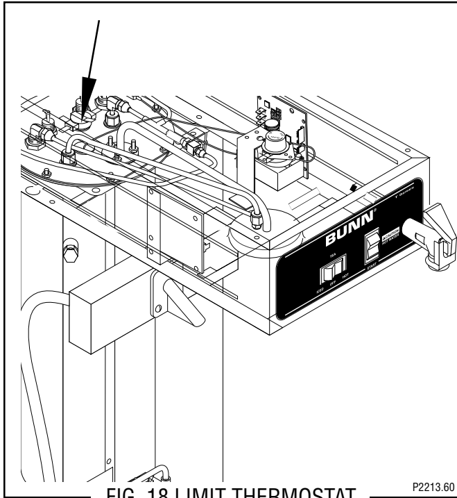
FIG. 18 LIMIT THERMOSTAT
