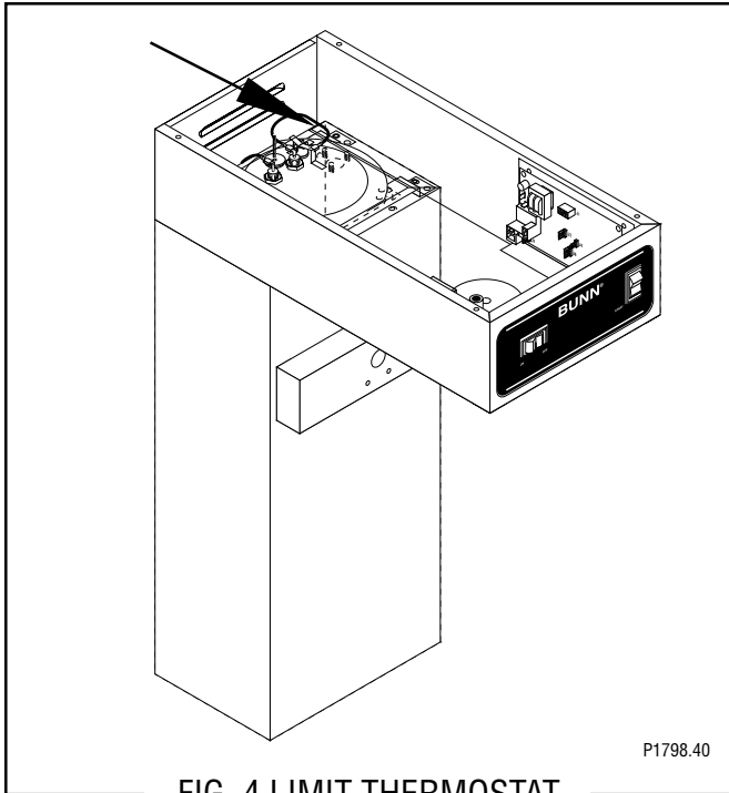
FIG. 4 LIMIT THERMOSTAT
