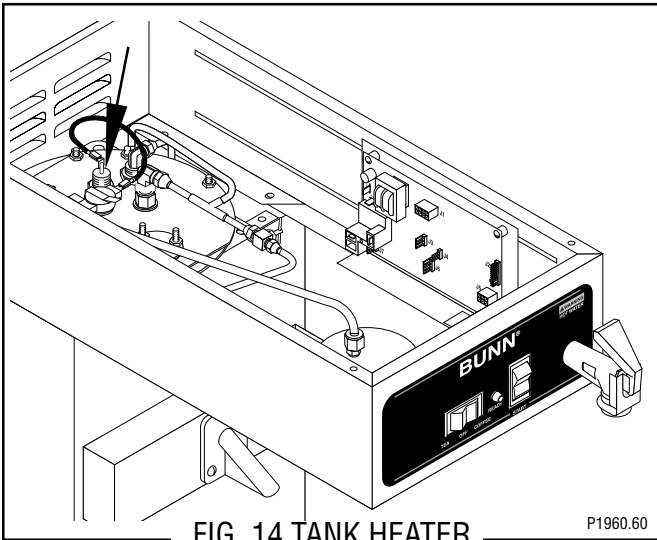
FIG. 14 TANK HEATER
