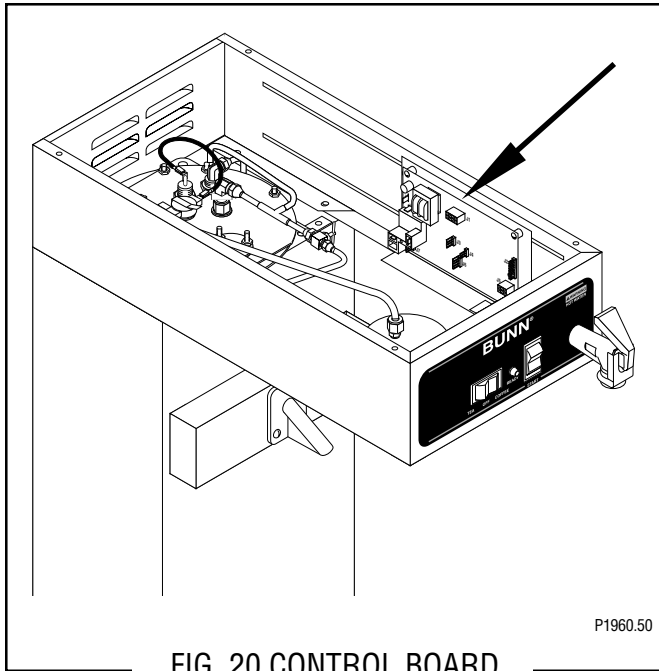
FIG. 20 CONTROL BOARD
