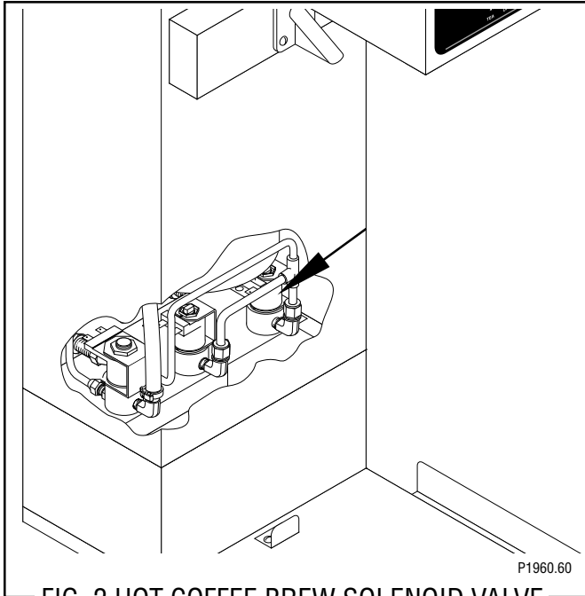
FIG. 2 HOT COFFEE BREW SOLENOID VALVE
