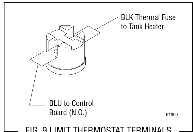
FIG. 9 LIMIT THERMOSTAT TERMINALS
