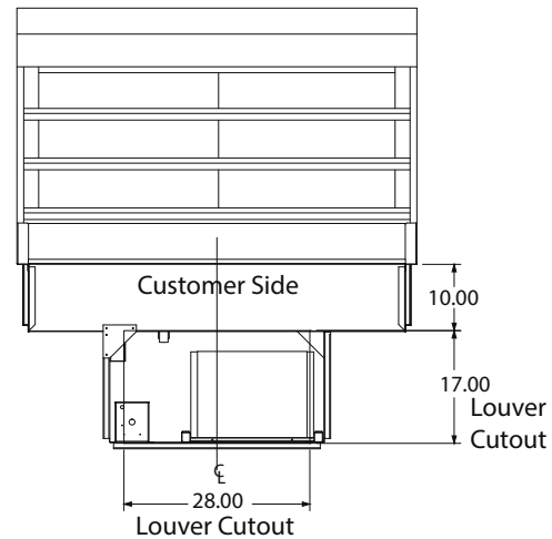
Customer Side Louver Cutout Dimensions
