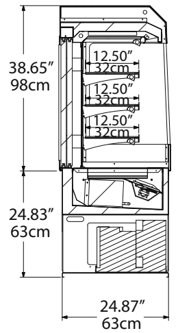
Left Section View, ASM-36, ASM-48
