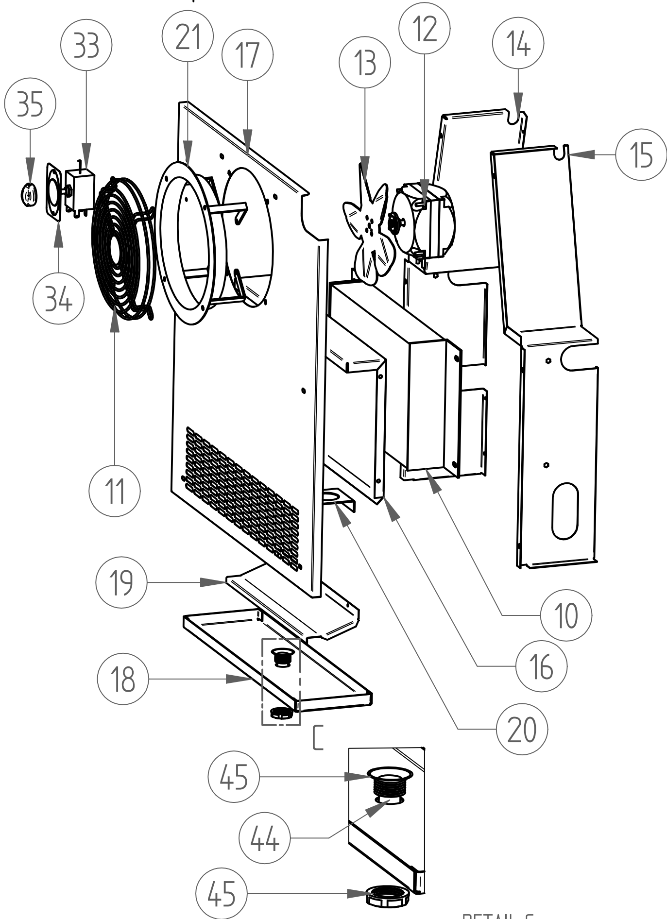
DETAIL C
