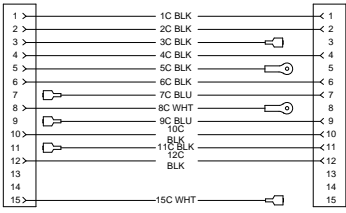
Computer harness
