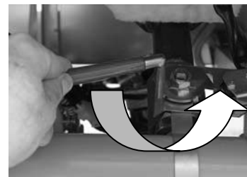
Move the red drain valve handle into the open position (right).
