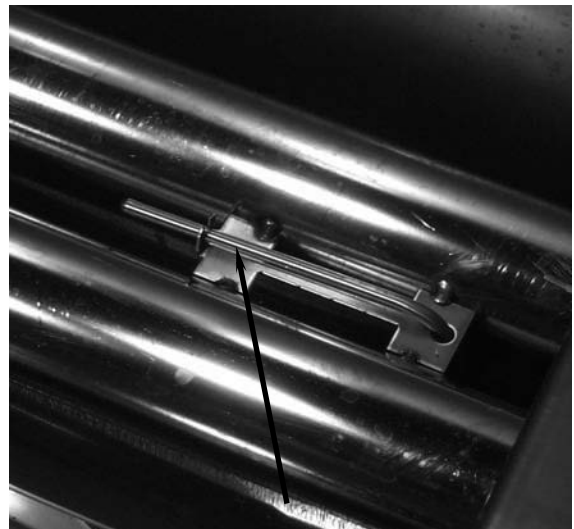
Electronic thermostat probe in frypot (arrow).
