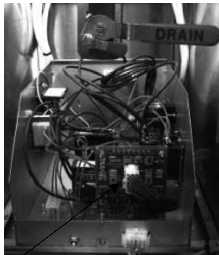
Fig: 10-7 The interface board is in the contactor box in the submarine fryer.
