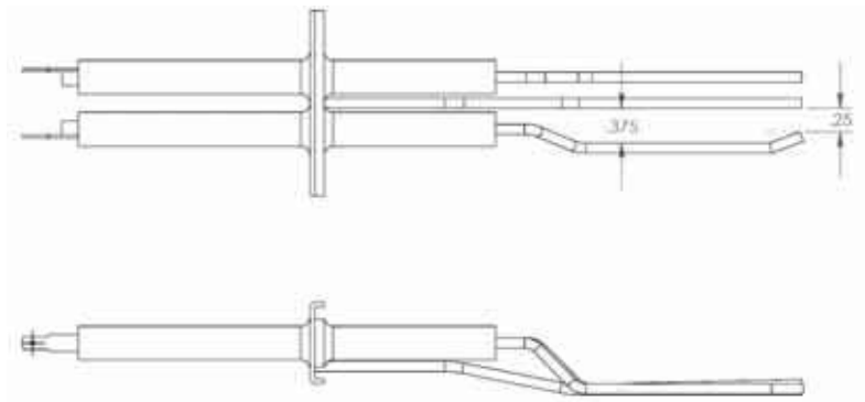
Figure 2A. The 1/4" space require between Igniter E1578 and ground
