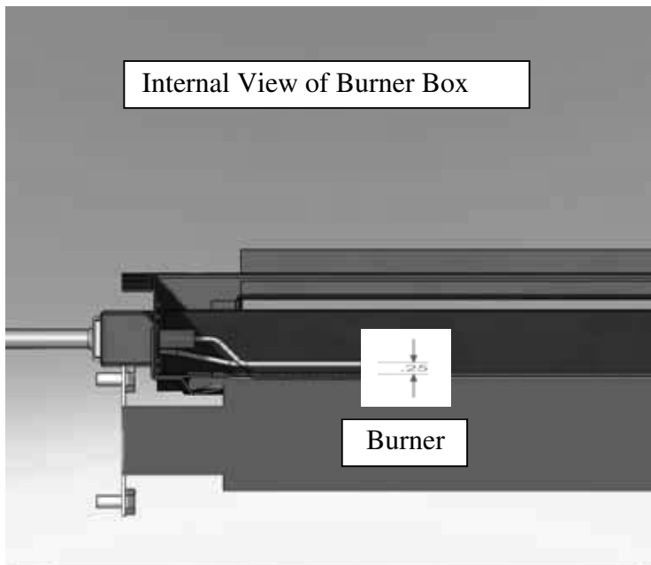
Figure1A. The Igniter E1578 and ground should be 1/4" away from the burner
