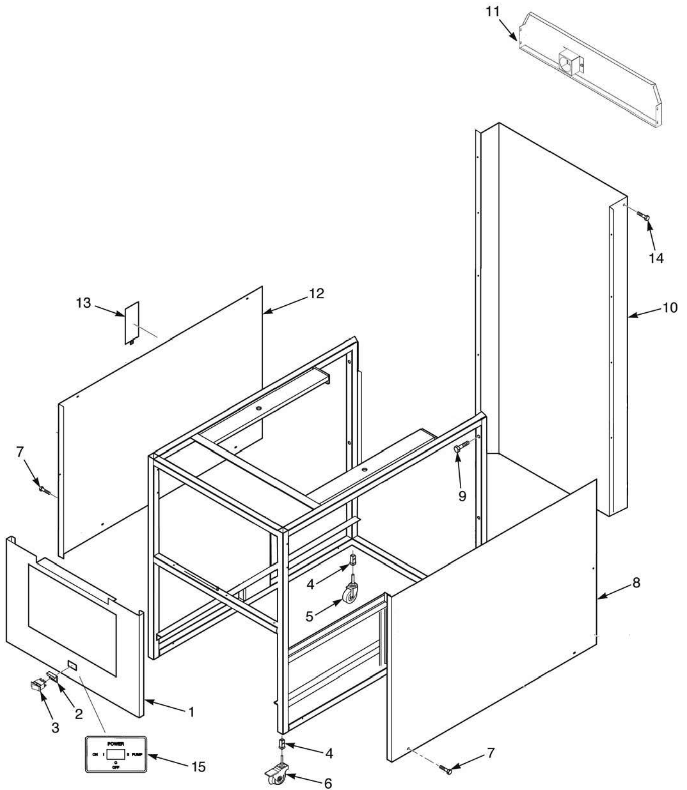
Figure 3-1. Frame and Cover Assembly
