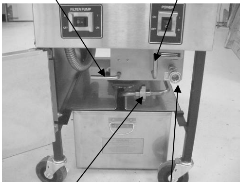
FILTER UNION FEMALE QUICK-DISCONNECT
