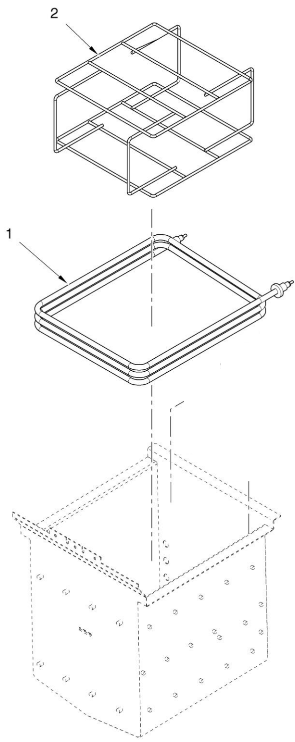
Figure 3-7. Electric Heater
