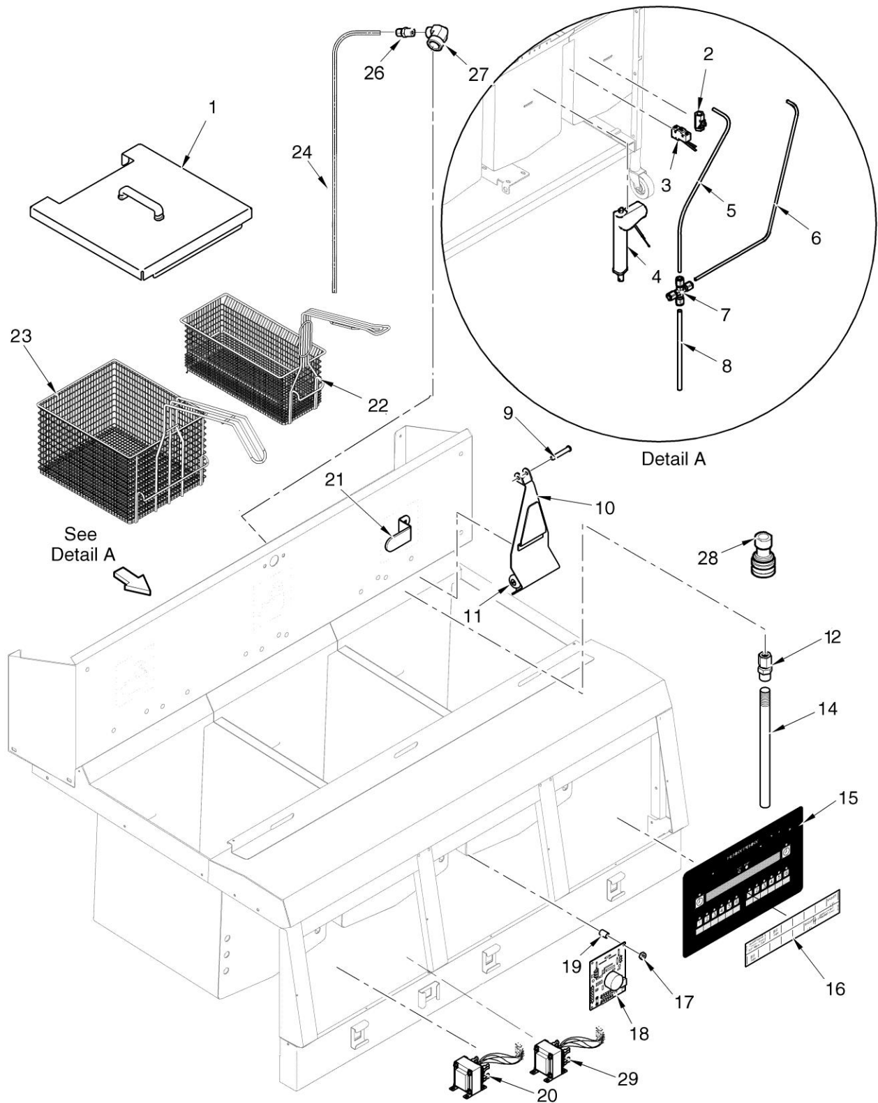
Figure 3-9. Autolift Feature
