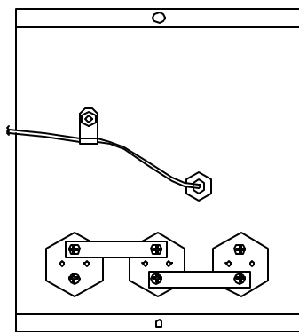
Heater Bus Bar (3 Phase) 5700-000-32-14
