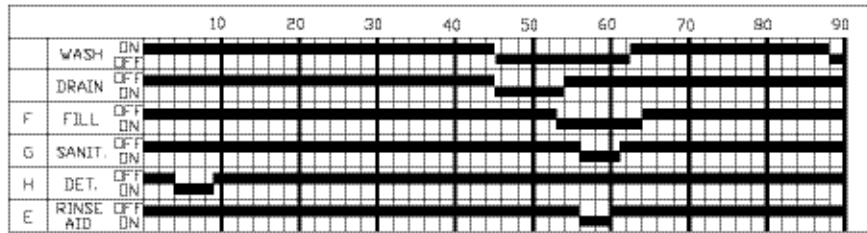
TIMING CHART
