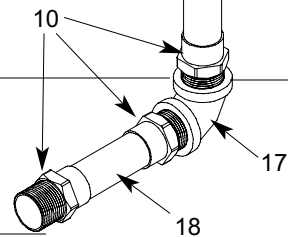
Lower Outlet Plumbing Assembly 5700-003-20-36
