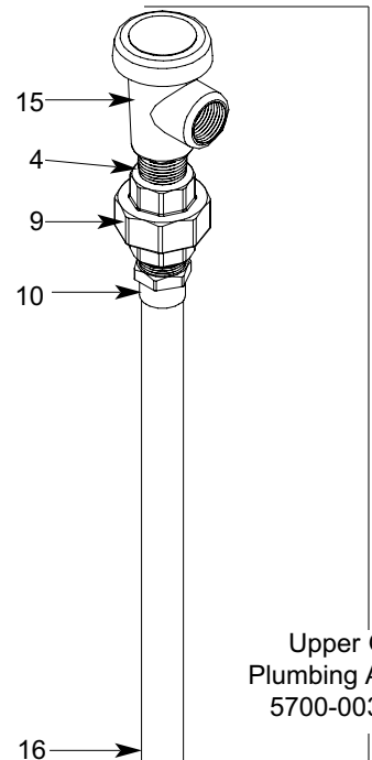
TEMPSTAR/TEMPSTAR SDS OUTLET PLUMBING
