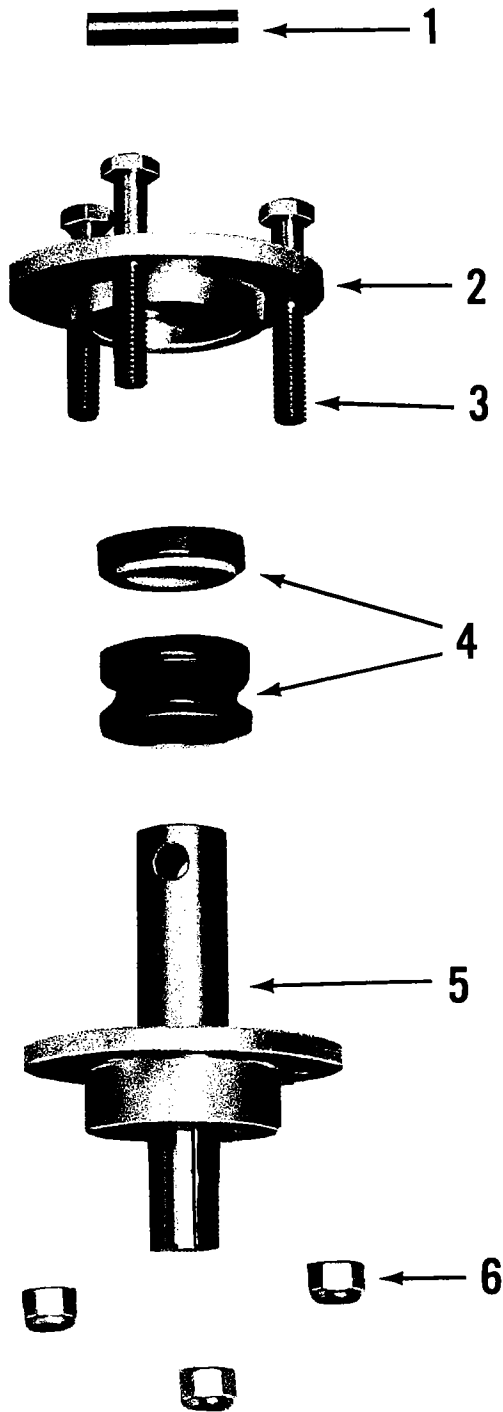
FIG. 12 LOWER BEARING & SEAL ASSEMBLY.
