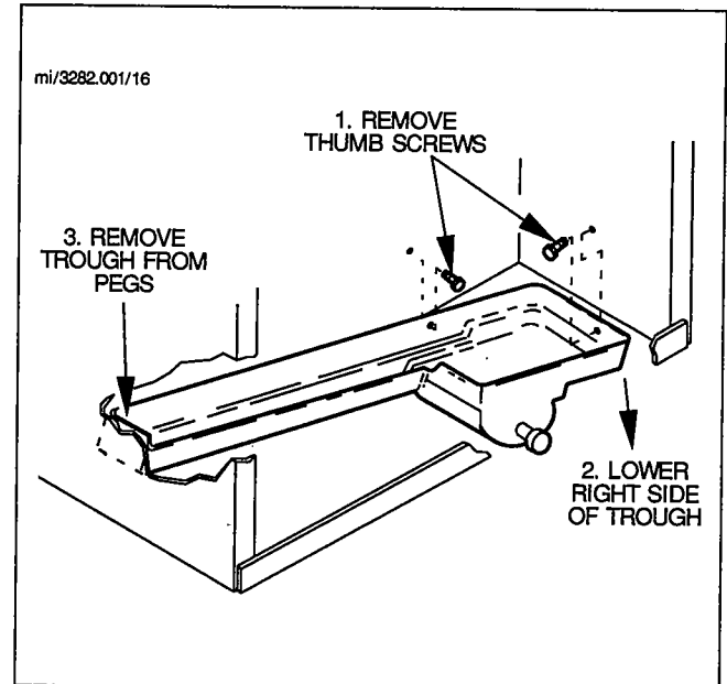
FIGURE 16. WATER TROUGH REMOVAL (G200 MODELS SHOWN)
