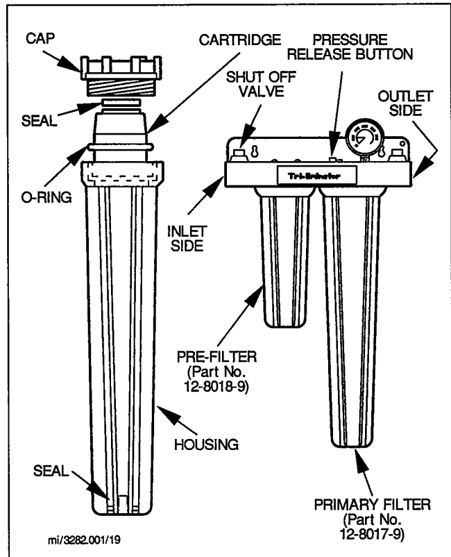
FIGURE 19. WATER FILTRATION
