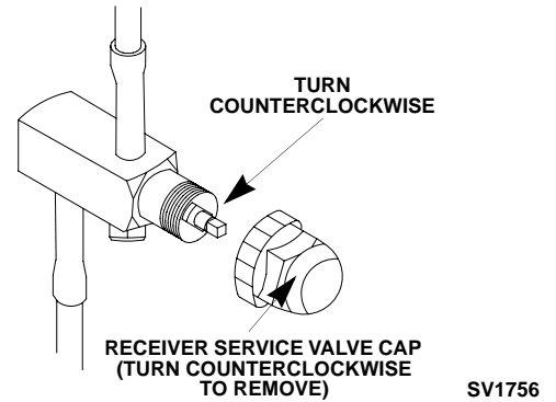
Open Receiver Service Valve
