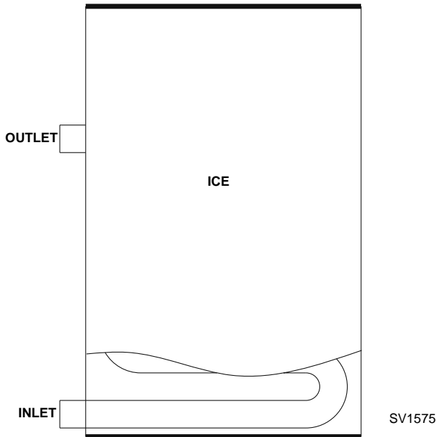
Figure 7-9. Extremely Thin Ice Formation at Evaporator Inlet
