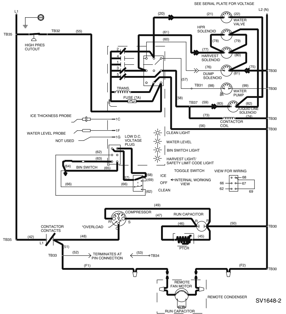
Figure 6-9. Remote — Refrigeration System Start-Up
