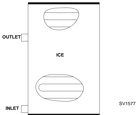
Figure 7-10. Spotty Ice Formation
