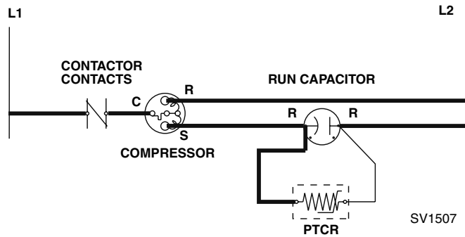
Figure 6-16. After Start-Up (Current Flows Through Run Capacitor)
