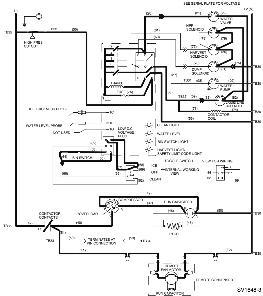
Figure 6-10. Remote — Pre-Chill
