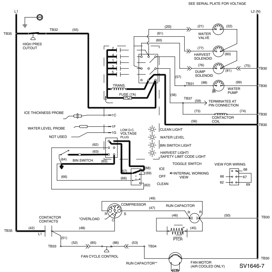
Figure 6-7. Self-Contained — Automatic Shut-Off
