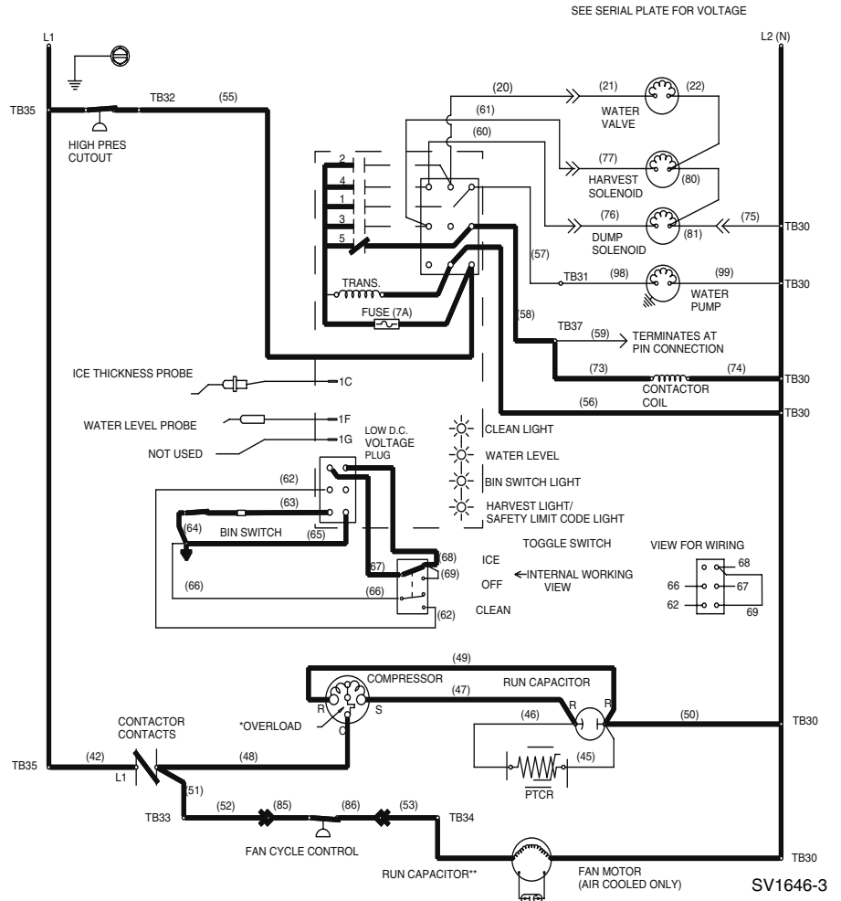
Figure 6-3. Self-Contained — Pre-Chill
