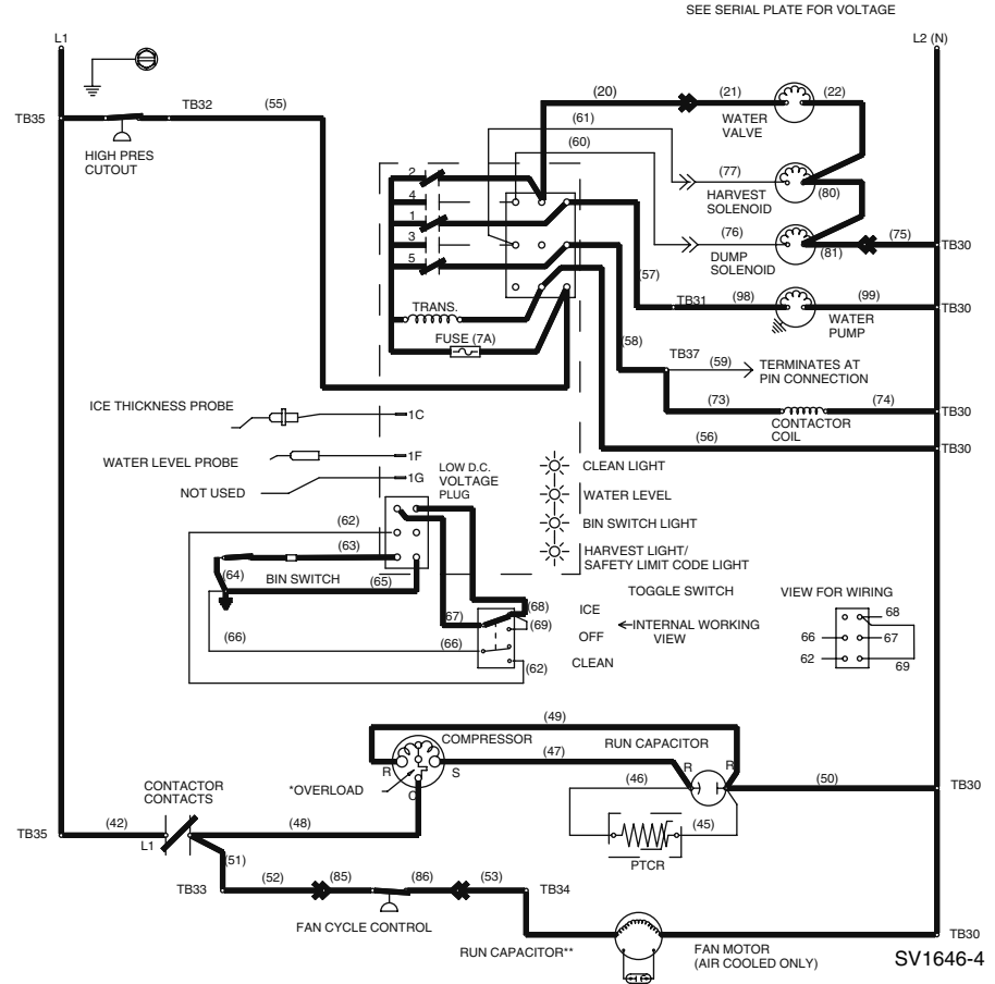
Figure 6-4. Self-Contained — Freeze
