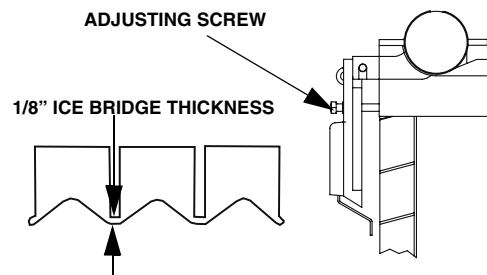
Figure 6-21. Ice Thickness Check
