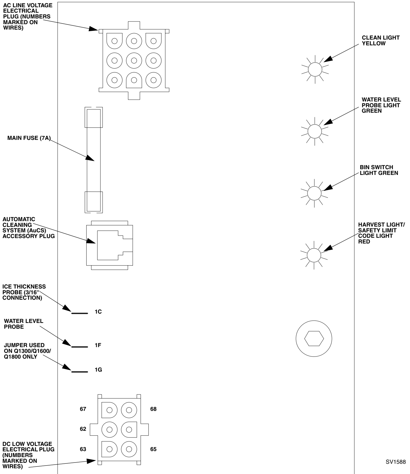
Figure 6-19. Control Board
