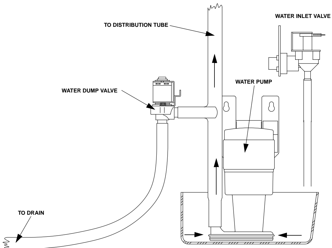
Figure 5-1. Water Flow Over the Evaporator
