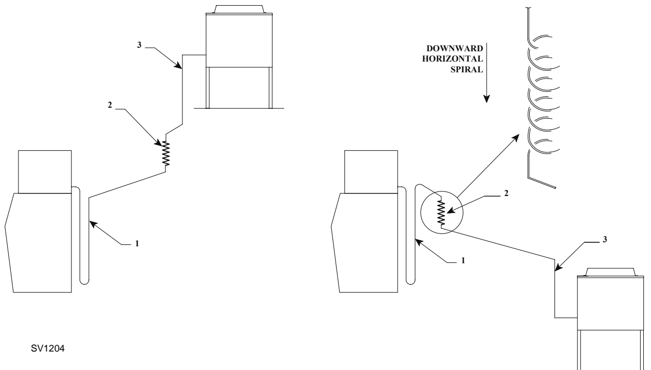
Figure 2-5. Routing Line Sets
