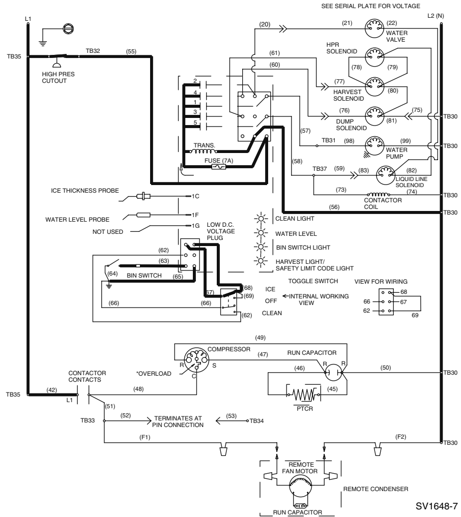
Figure 6-14. Remote — Automatic Shut-Off
