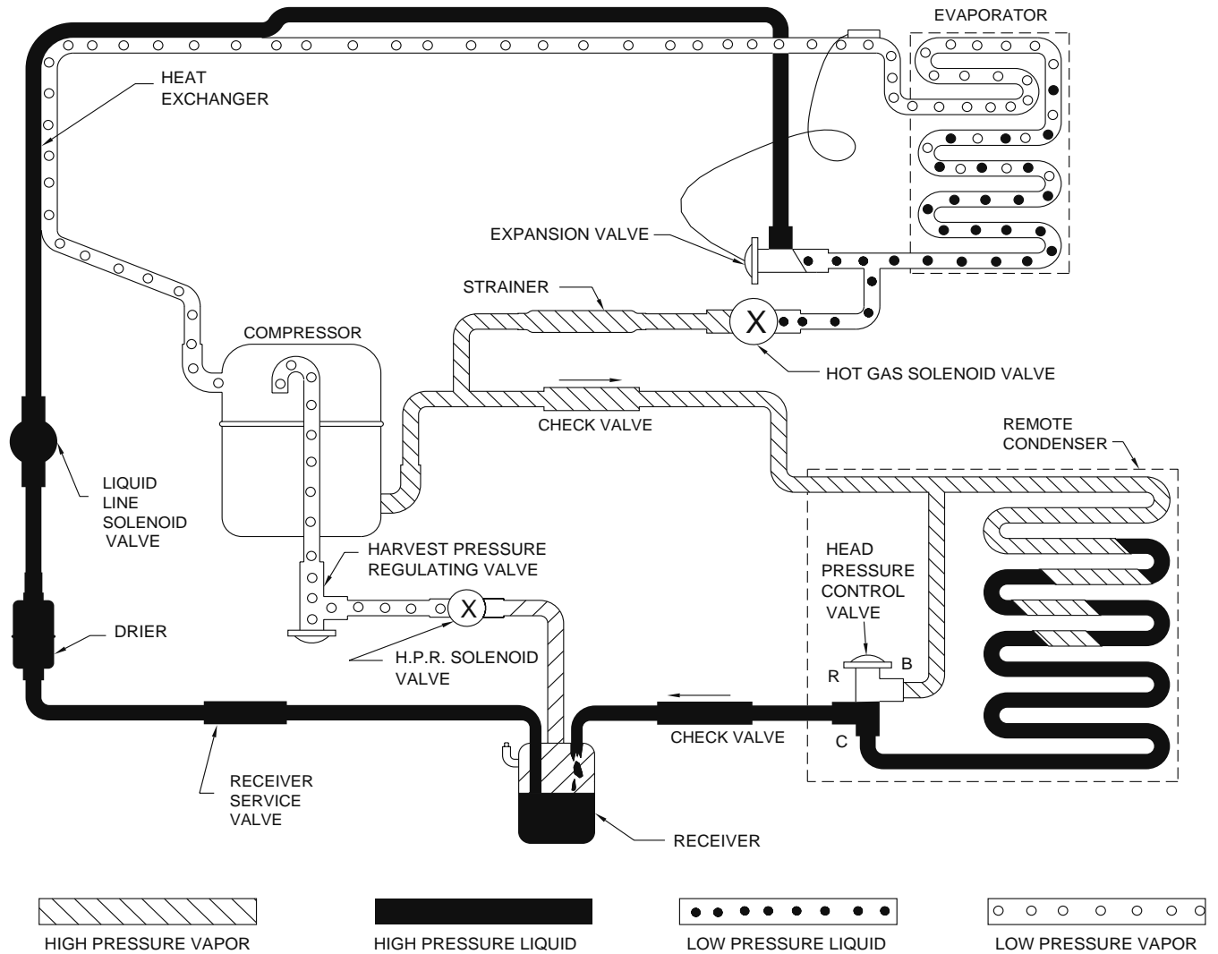
Figure 7-3. Remote Pre-Chill and Freeze Cycle (Models Q450/Q600/Q800/Q1000)
