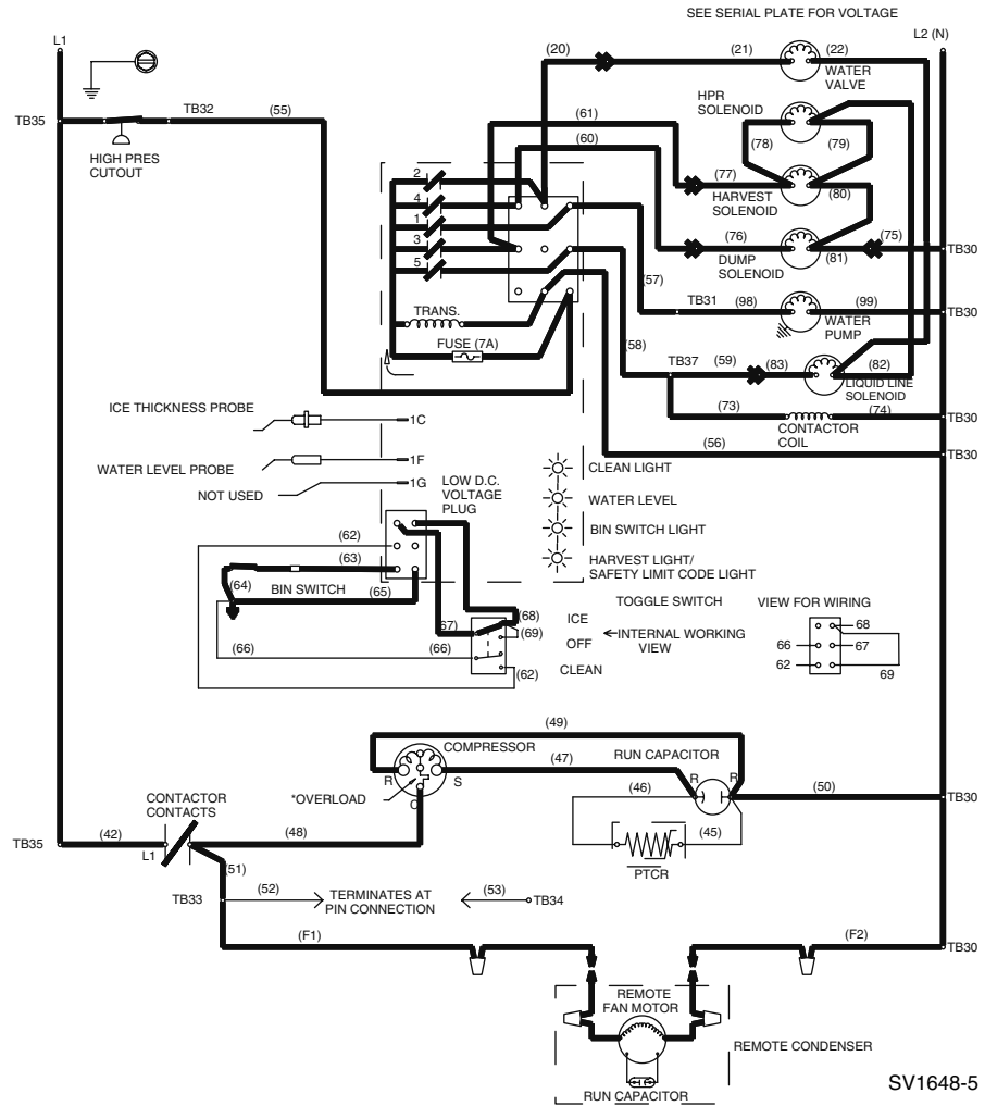
Figure 6-12. Remote — Water Purge
