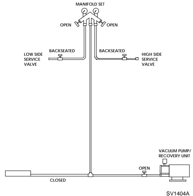
Figure 7-14. Recovery/Evacuation Connections
