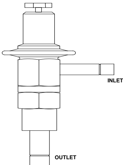
Figure 7-13. H.P.R. Valve
