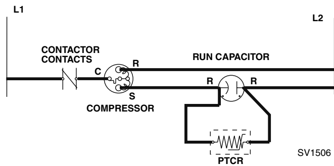
Figure 6-15. During Start-Up (First .25 - 1.0 Seconds)
