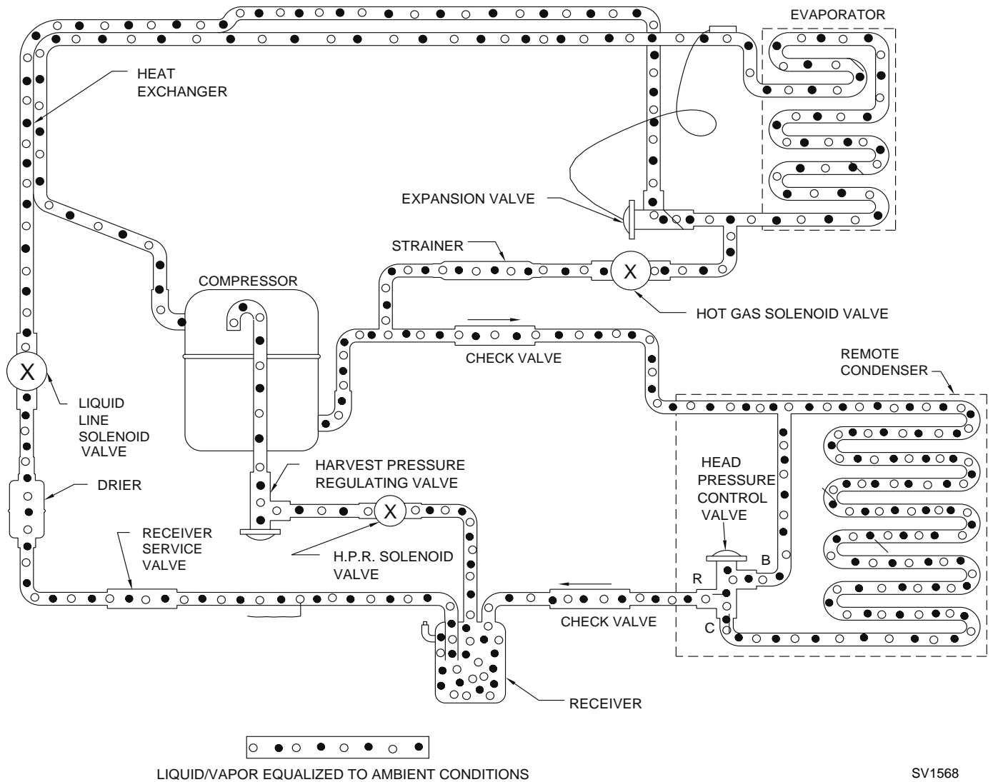
Figure 7-5. Remote Automatic Shut-Off (Models Q450/Q600/Q800/Q1000)
