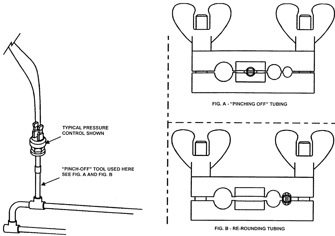
Figure 7-18. Using Pinch-Off Tool
