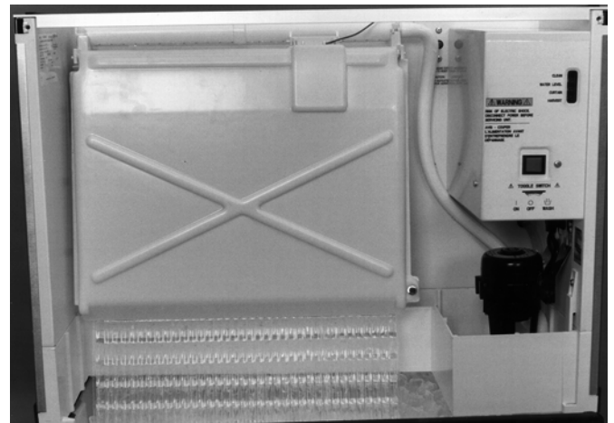
Figure 3-7. Automatic Shut-Off (Typical Q450 Shown)
