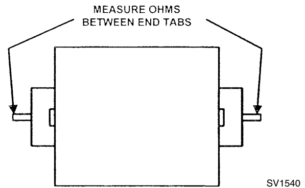
Figure 6-17. Manitowoc PTCR's 8505003 & 8504993
