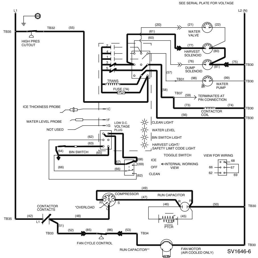
Figure 6-6. Self-Contained — Harvest
