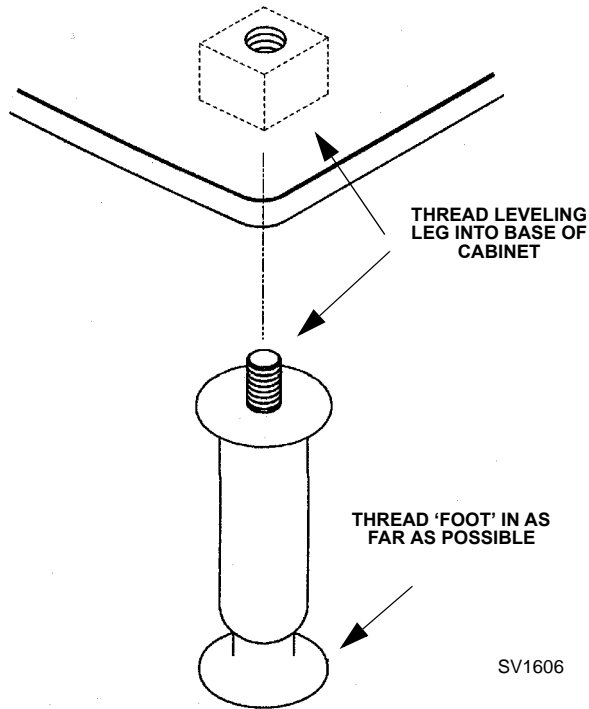
Figure 2-1. Leveling Leg and Foot
