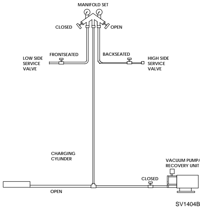
Figure 7-15. Charging Connections
