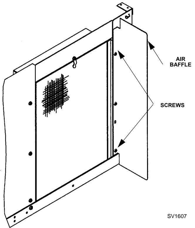
Figure 2-2. Air Baffle
