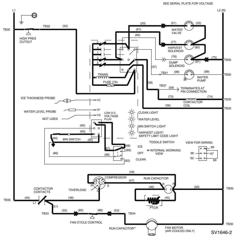
Figure 6-2. Self-Contained — Refrigeration System Start-Up
