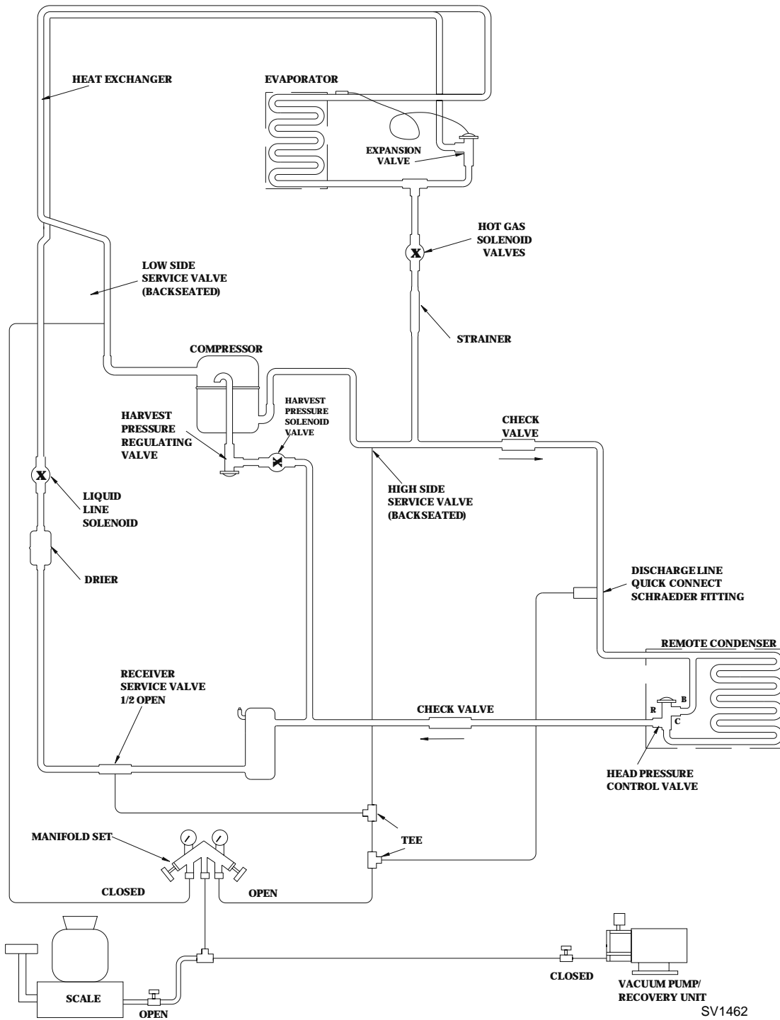
Figure 7-17. Remote Charging Connections
