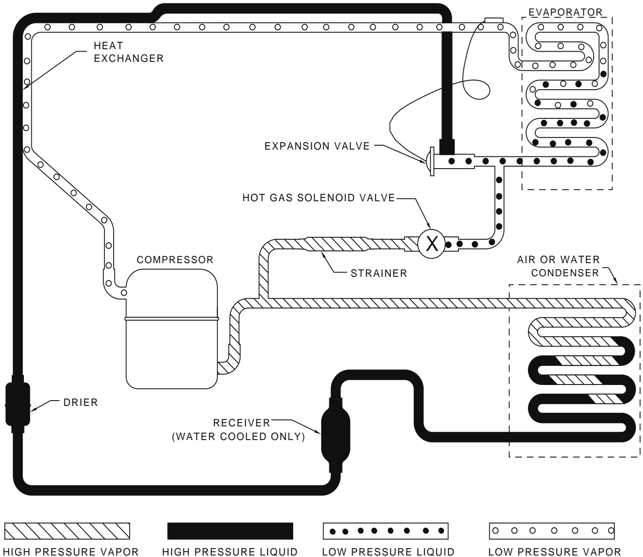
Figure 7-1. Self-Contained Prechill and Freeze Cycle (Models Q200/Q280/Q320/Q370/Q420/Q450/Q600/Q800/Q1000)
