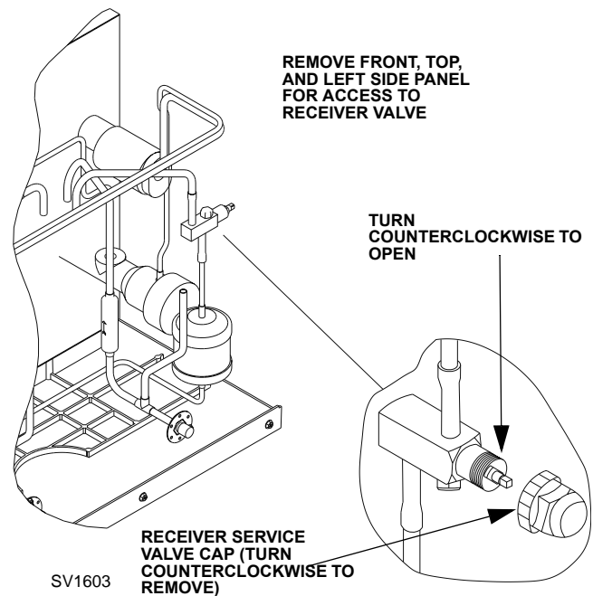
Figure 2-9. Backseating the Receiver Service Valve
