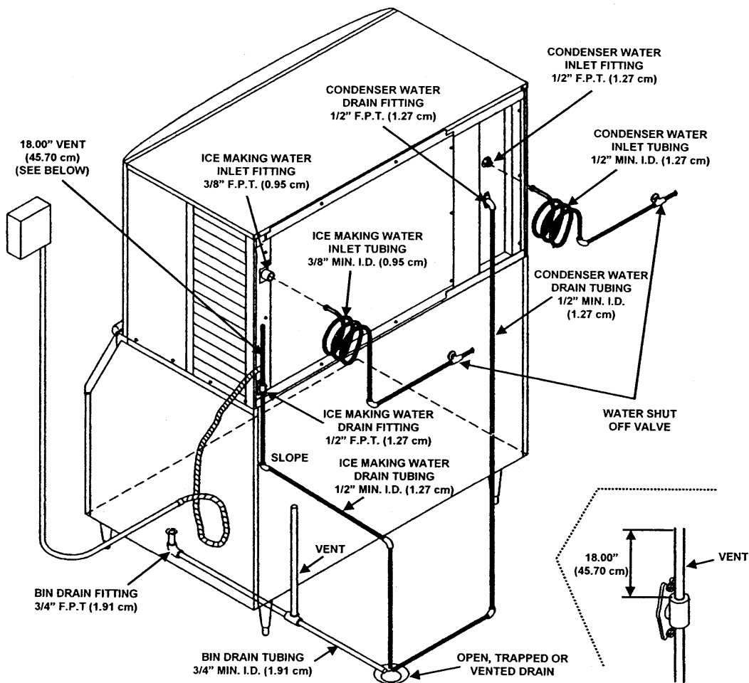
Figure 2-3. Typical Water Supply Drain Installation
