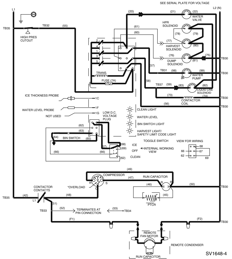
Figure 6-11. Remote — Freeze
