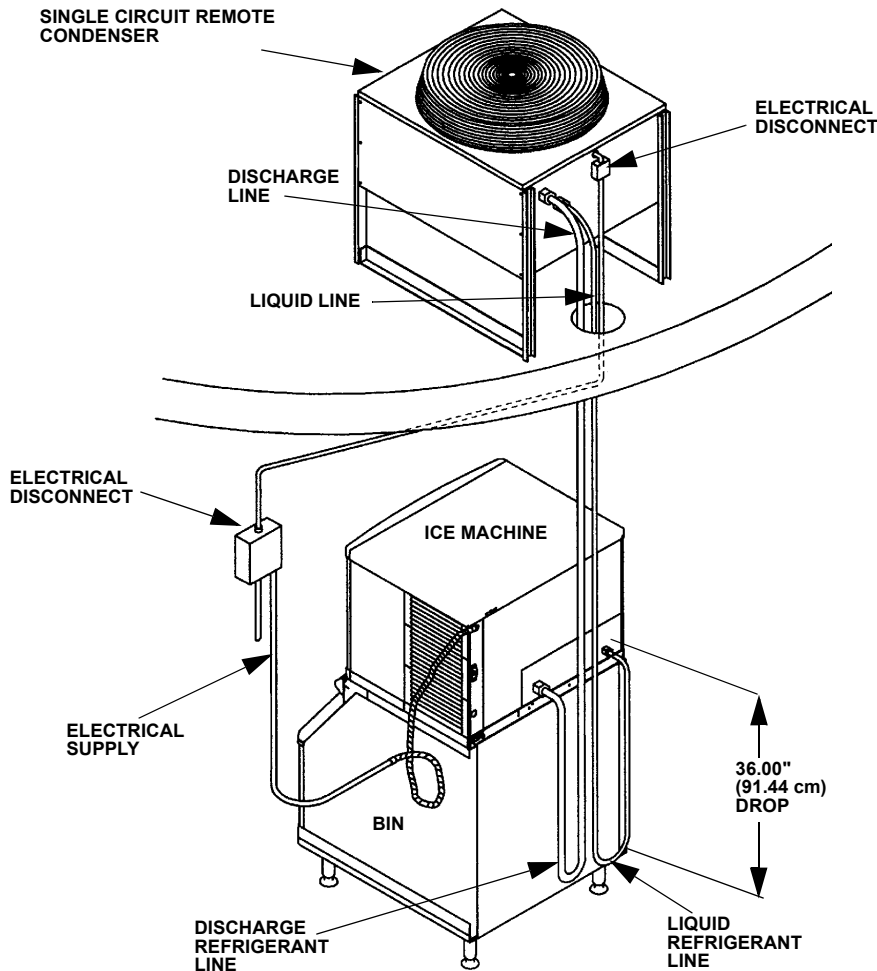
Figure 2-10. Typical Single Circuit Remote Condenser Installation
