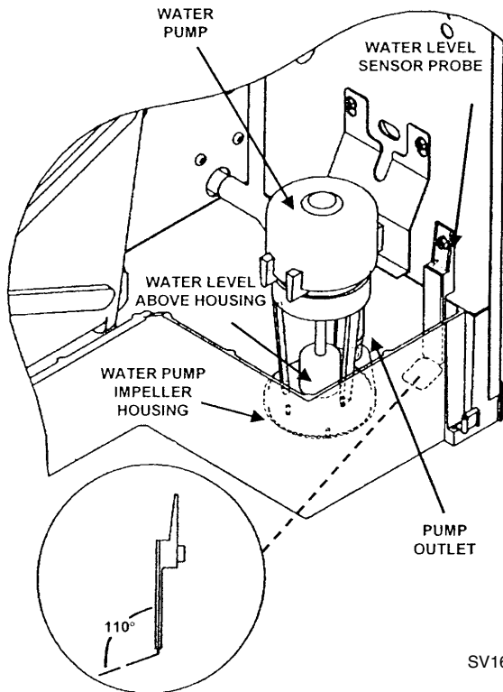
Figure 6-25. Freeze Cycle Water Level Setting
