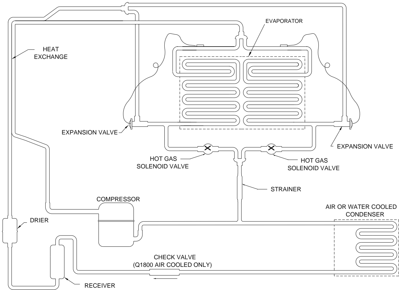
Figure 7-6. Q1300/Q1600/Q1800 Self-Contained Air- or Water-Cooled Models
