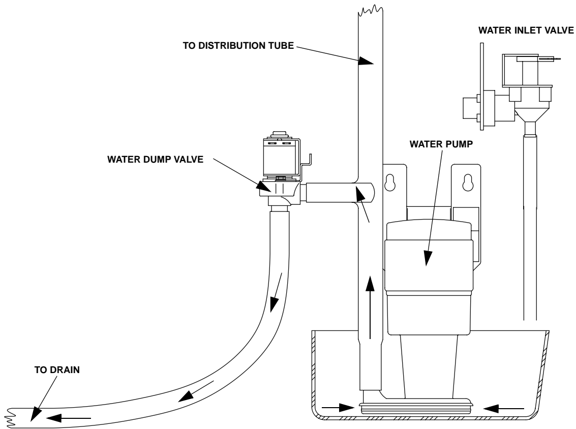
Figure 5-2. Water Flow Down the Drain
