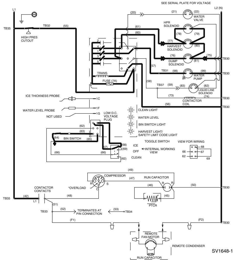
Figure 6-8. Remote — Water Purge
