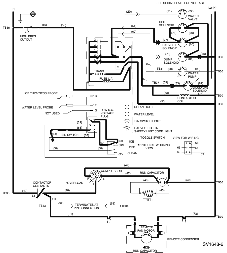
Figure 6-13. Remote — Harvest
