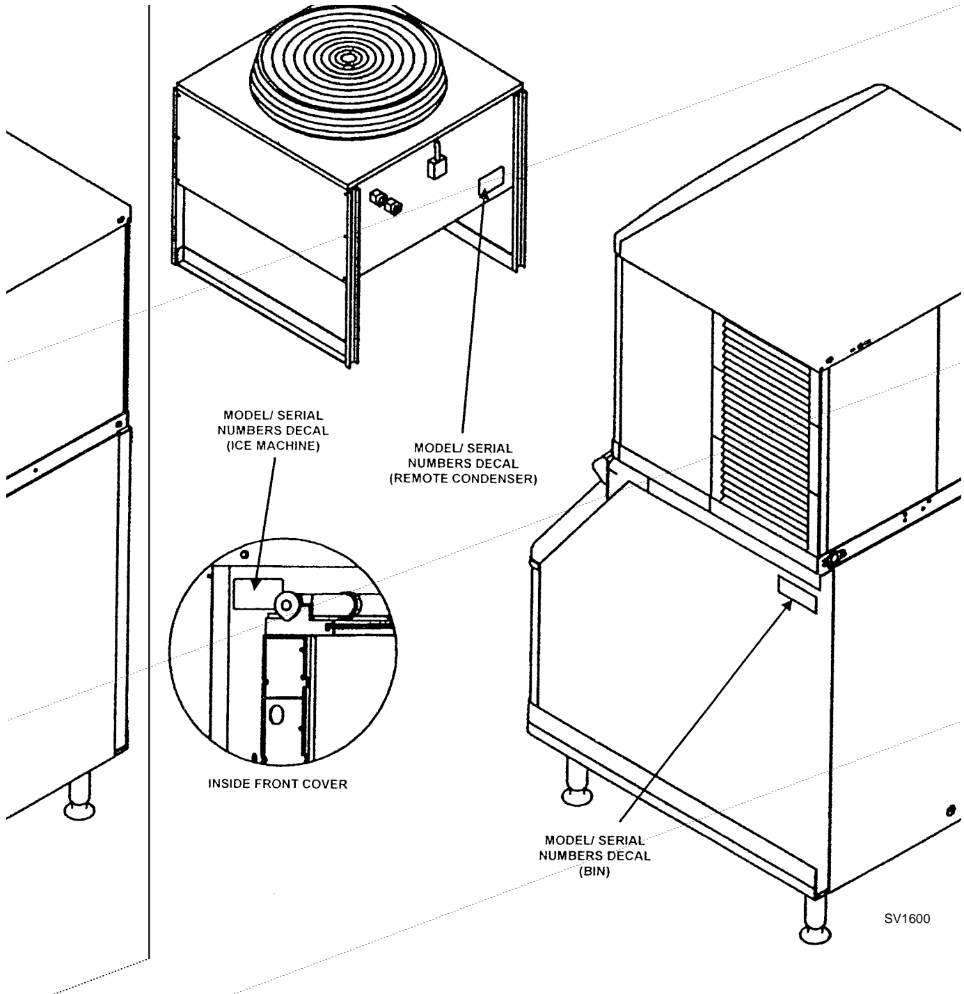
Figure 1-1. Model/Serial Number Location
