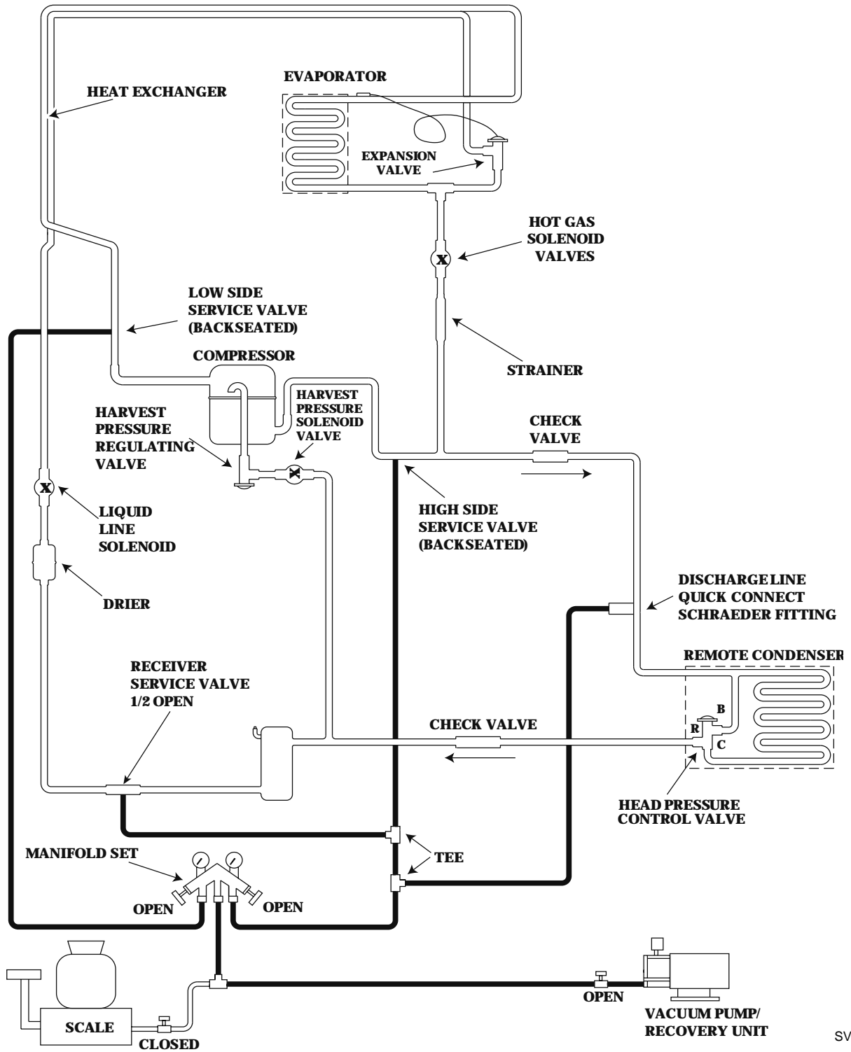
Figure 7-16. Recovery/Evacuation Connections
