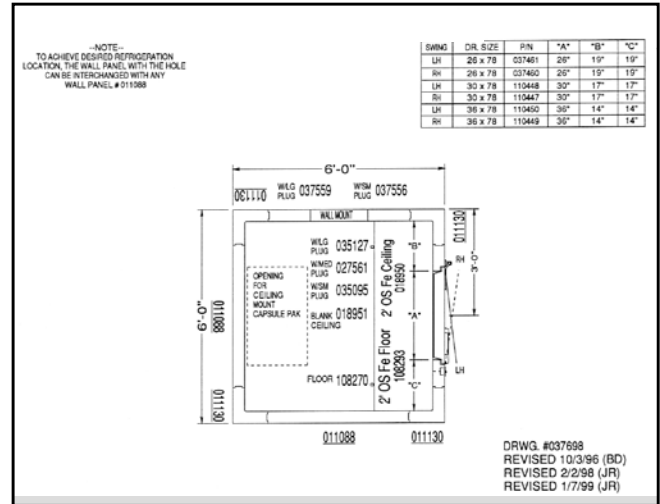
Construction Diagram
