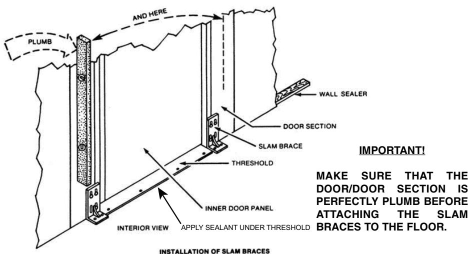
INSTALLATION OF SLAM BRACES
