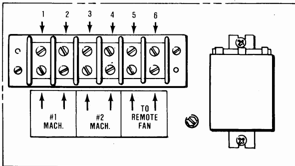
KCMR230 RELAY BOX
