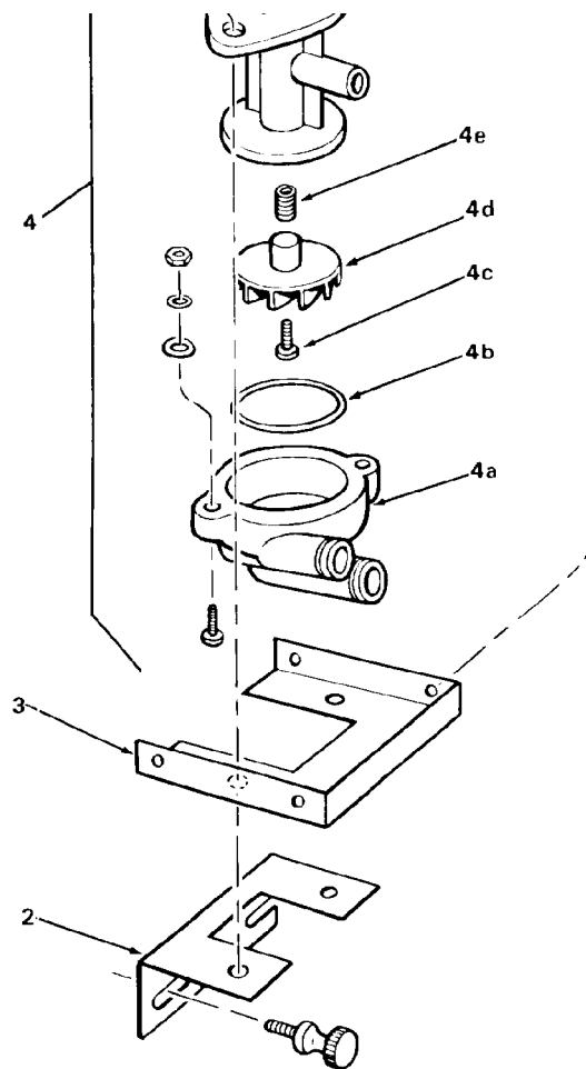
Figure 8-7. Water Pump, Bracket & Enclosure Assembly.
