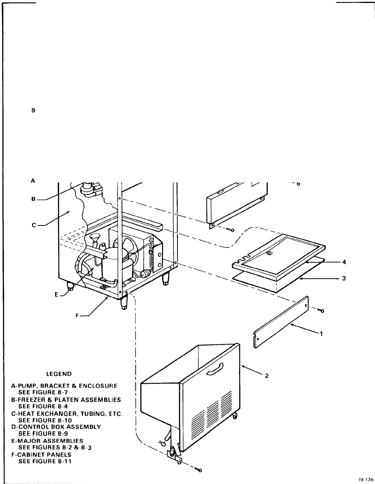
Figure 8-1. AC-20 Cabinet.
