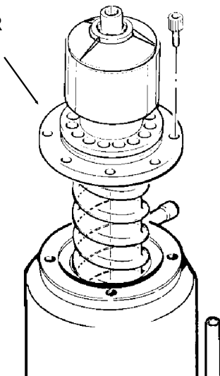
BREAKER AND AUGER ASSEMBLY
