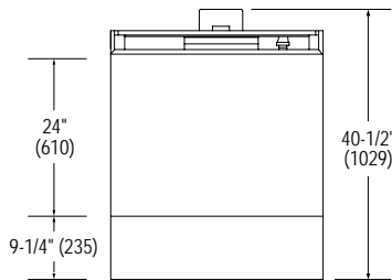
SIDE VIEW of Charbroiler/Griddle Oven-Base Models
