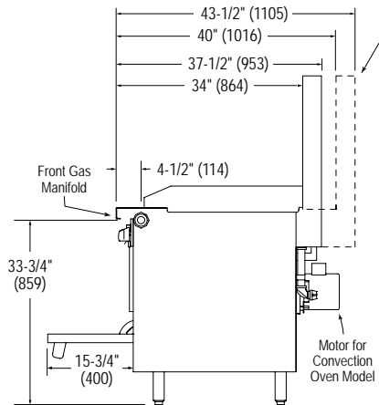
SIDE VIEW of Charbroiler/Griddle Oven-Base Models
