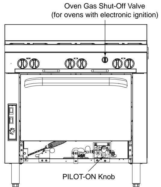
Controls for Ovens with Electronic Ignition
