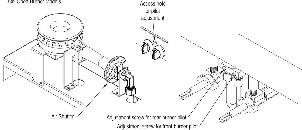
33K-Open-Burner Models
