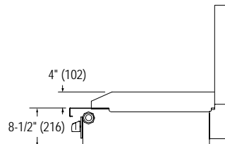
SIDE VIEW of Charbroiler/Griddle Modular-Base Models
