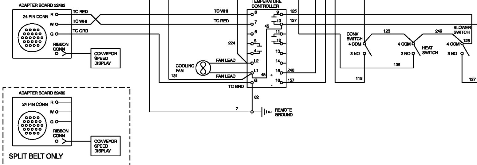
Fig. 6-2 - Wiring diagram, PS536GS Gas Oven 208/240V, 50/60 Hz, 1 Ph
