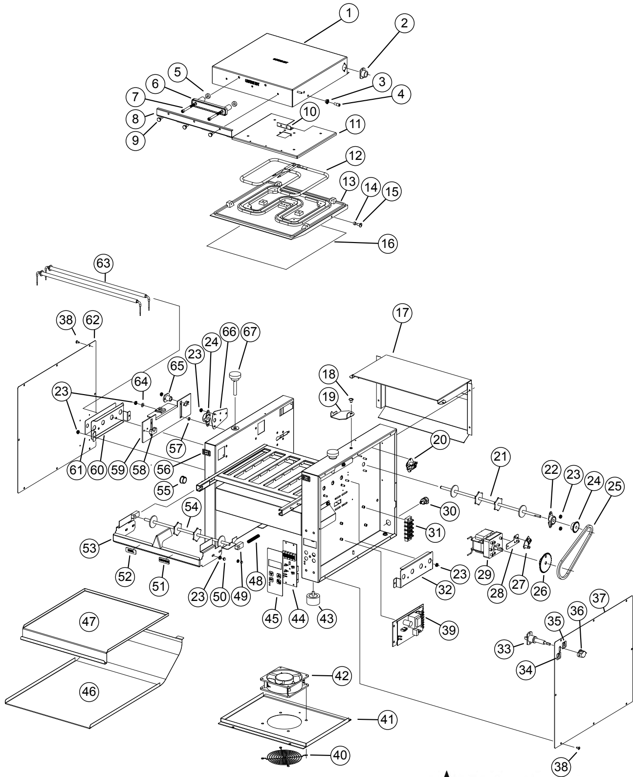
Model: HCTE13SW Contact Toasters w/electronic controls
