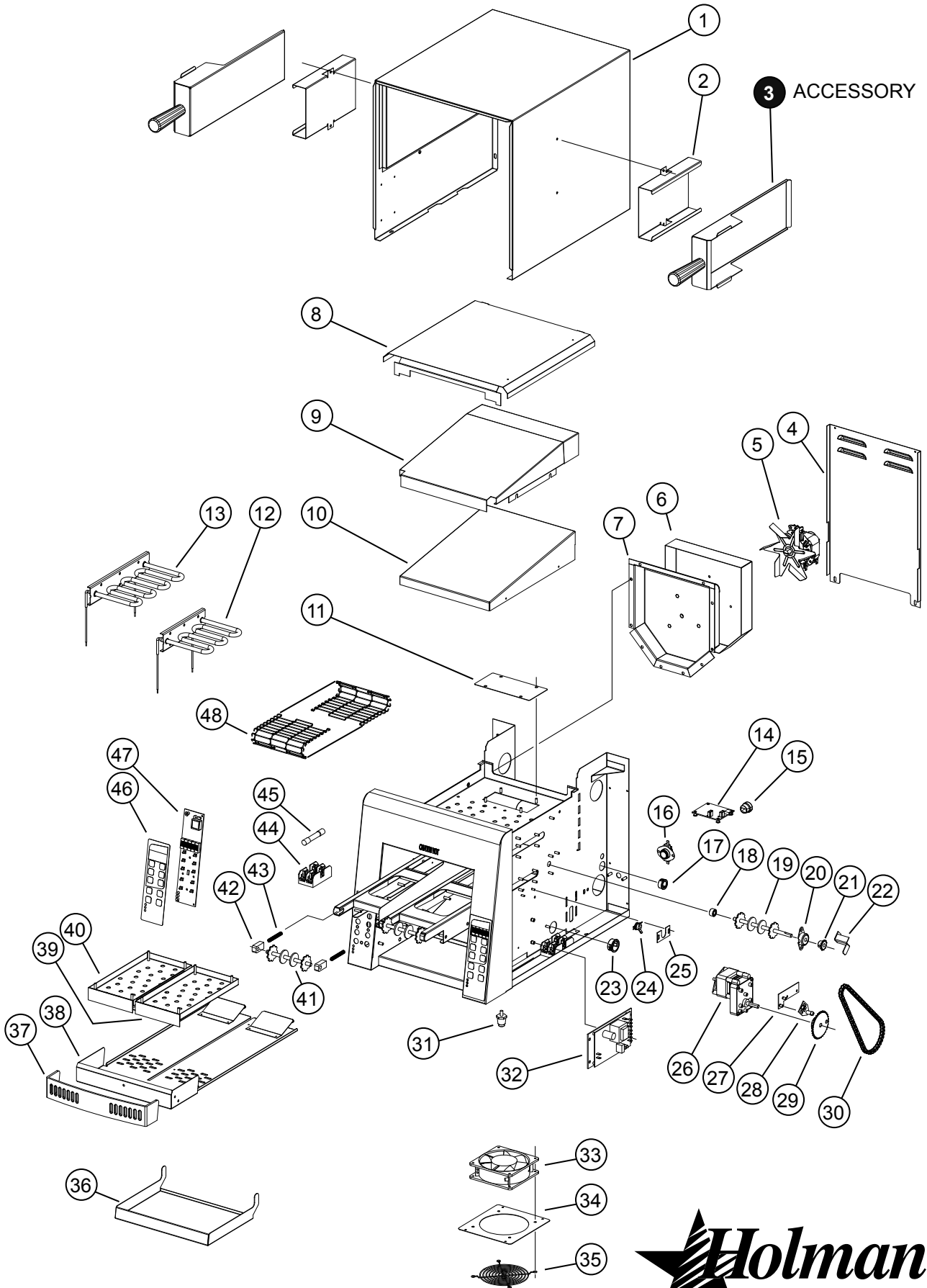
MODEL: IRCS2-SBD: Split Electronic Conveyor Toaster
