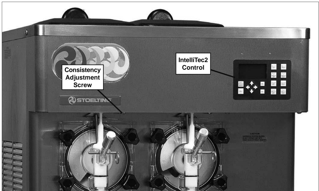
Figure 3-1 F122 Controls
