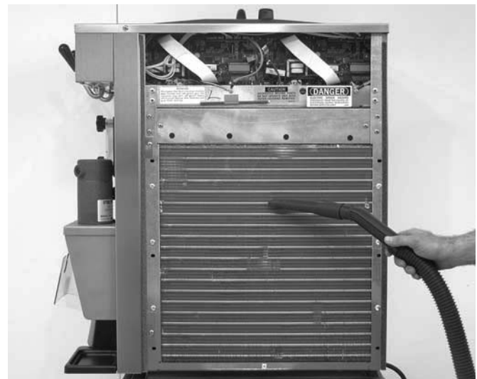
Figure 29. Cleaning Condenser
