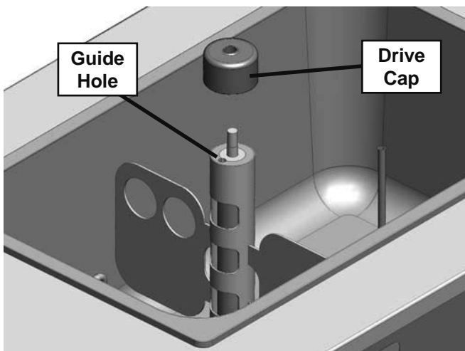
Figure 3-3 Hopper Agitator and Drive Cap
