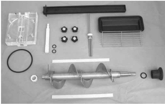
Figure 18. Exploded View of Auger (Front Door and Related Parts)
