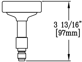
T&S NO. EB-1421 REGULAR SPRAY QUICK CONNECT (EPAAct2005 NON-COMPLIANT)
